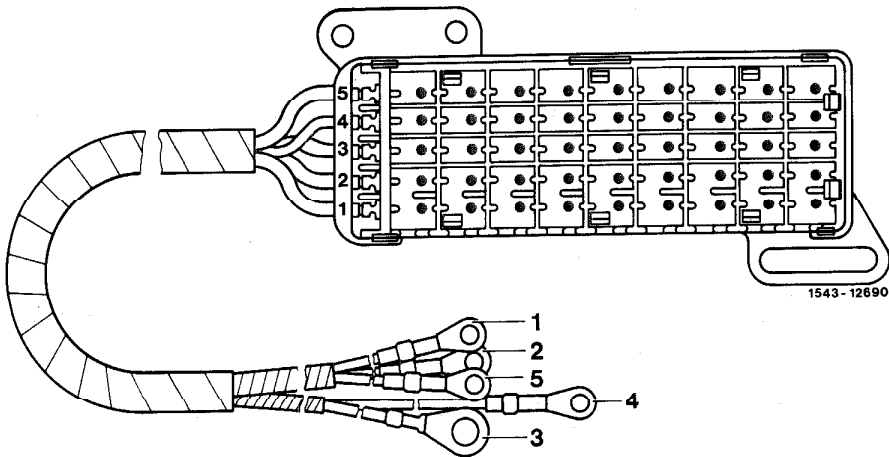
Allocation chart of connector block
